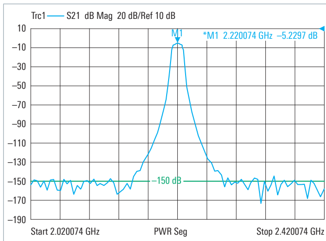
Filter measurement with segmented sweep.
