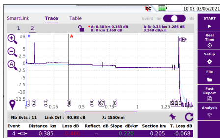
OTDR trace view
