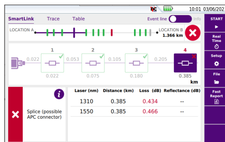
Smart Link Mapper view
