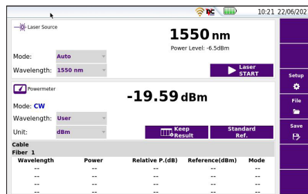
Built-in power meter and laser source
