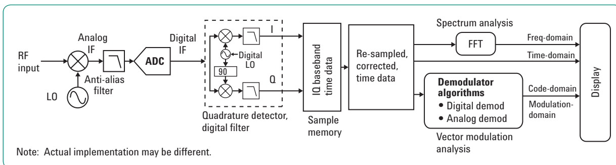
Figure 18. Simplified block diagram of a VSA measurement system with an RF front-end. For other front-ends, the VSA software will perform some functions not supported by the given front-end.
