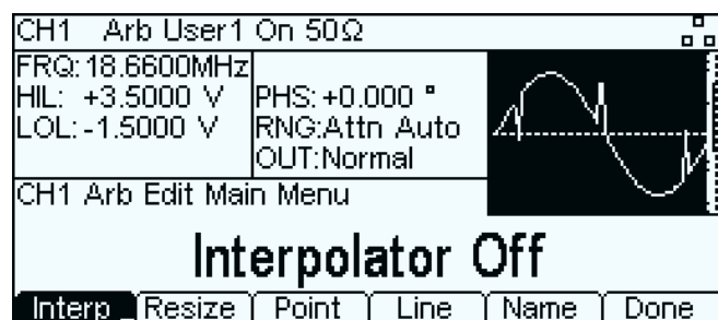
Arbitrary waveforms can be generated and edited within the instrument. Complex wave shapes are generated using the supplied PC software Waveform Manager Plus- see page 9
