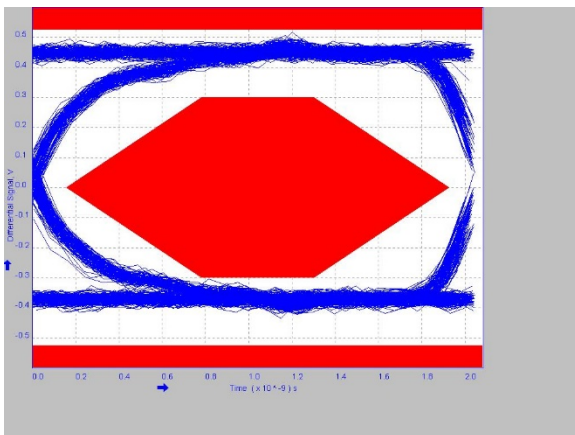
TDSUSB2 USB 2.0 Signal Quality Test Eye Diagram Captured with P6780 Differential Digital Probe using iCapture Analog MUX
