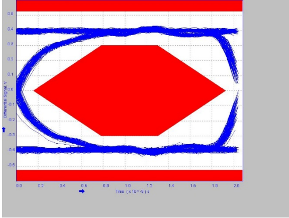
TDUSB2 USB 2.0 Signal Quality Test Eye Diagram Captured with P7330 3.5 GHz Differential Probe
