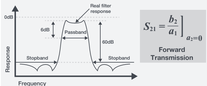
FIGURE 14. Swept frequency transmission measurement example of a passive filter.
