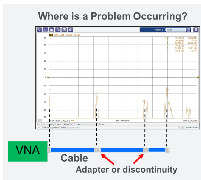
FIGURE 16. VNAs mathematically convert swept frequency measurements into the time domain. The measurements can be useful for locating impedance mismatches or faults in the line.
