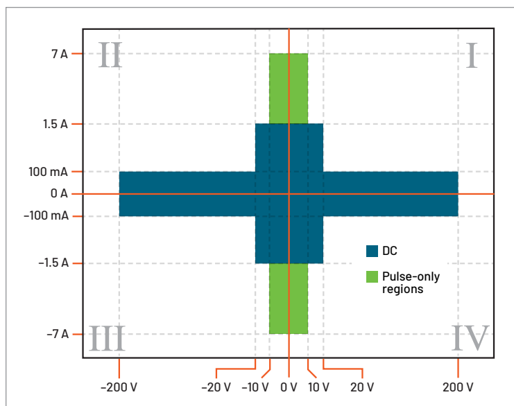
Figure 15: MSMU200-2 Power Envelope
