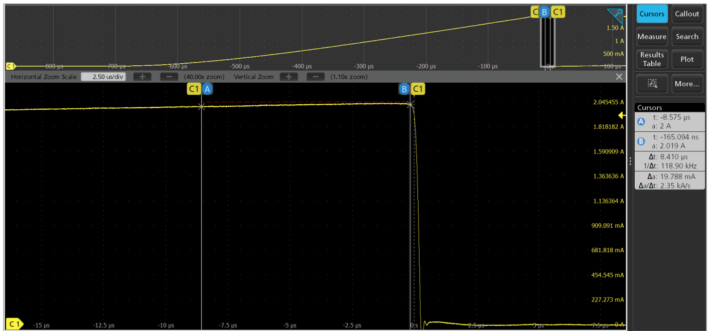
Figure 10: MPSU50-2ST OCP Response Time &lt;50usec
