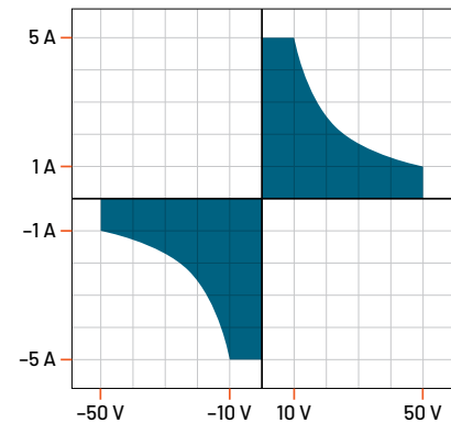
Figure 16: MPSU50-2ST Power Envelope
