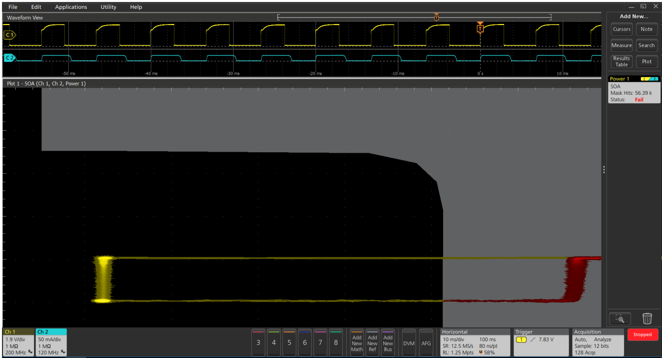
Figure 6: Safe Operating Area (SOA) plot with mask helps verify the switching devices are staying within their SOA envelope under changing operating conditions.
