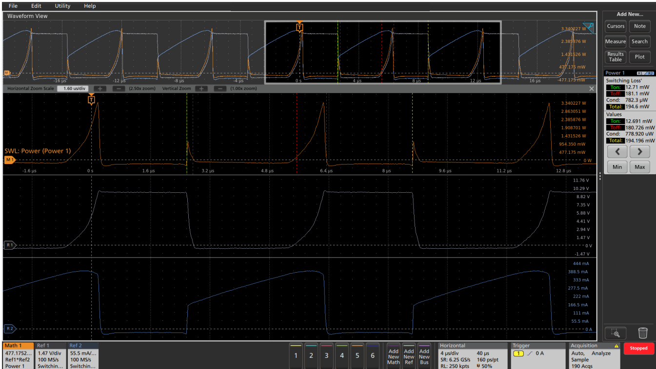
Figure 4: Switching Loss shows power dissipation in a FET. Waveforms are annotated with color-coded markers showing the measurement regions for T_{on} , T_{off} , and Total cycle, corresponding to values in the results badge. Controls in the results badge let you easily traverse from cycle to cycle.
