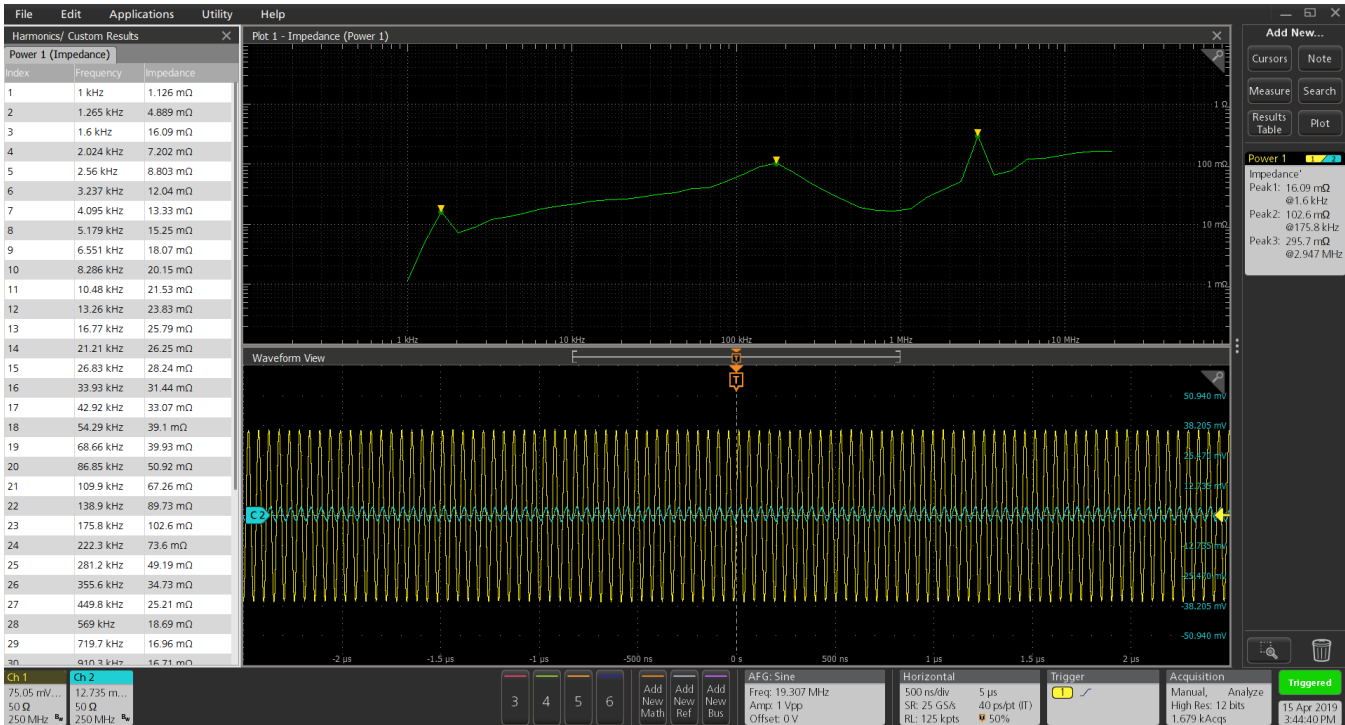
Figure 19: Impedance measurement with results table and results badge showing values for the peak impedance points.
