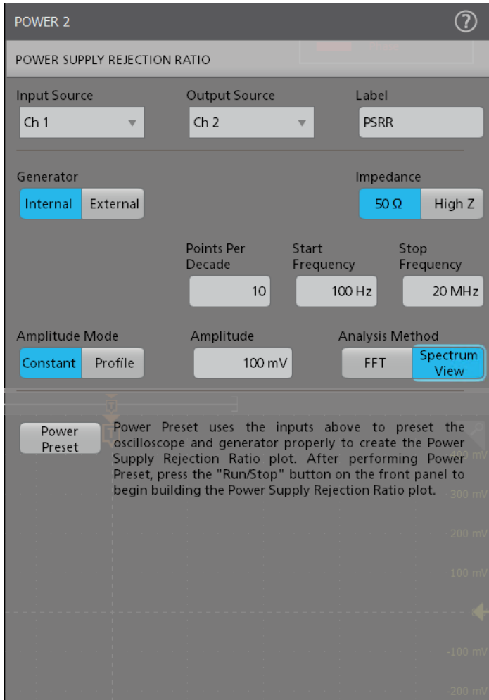
Figure 18: Control loop response and Power supply rejection ratio measurement allow you to set START and STOP frequencies of default internal AFG or external AFG31000 series. They also allow you to select constant/amplitude profile, impedance, and points per decade for better plot rendering
