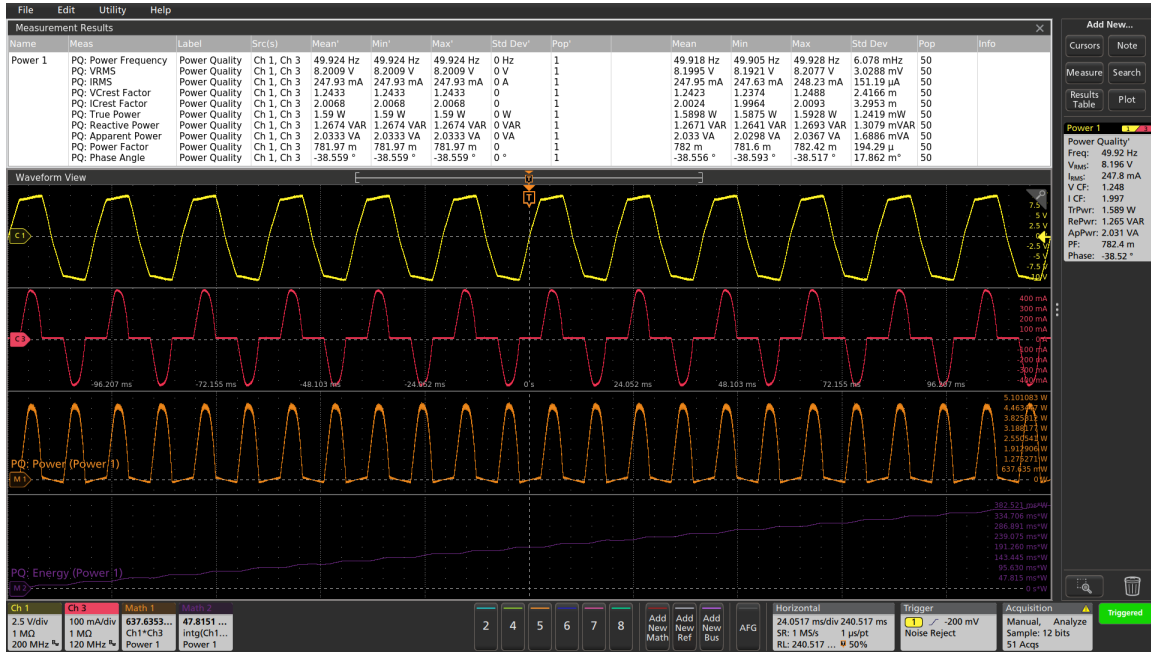
Figure 1: Power Quality measurements deliver information in multiple formats. Numerical results (upper right), tables (upper), and instantaneous power waveform and energy plots (lower)
