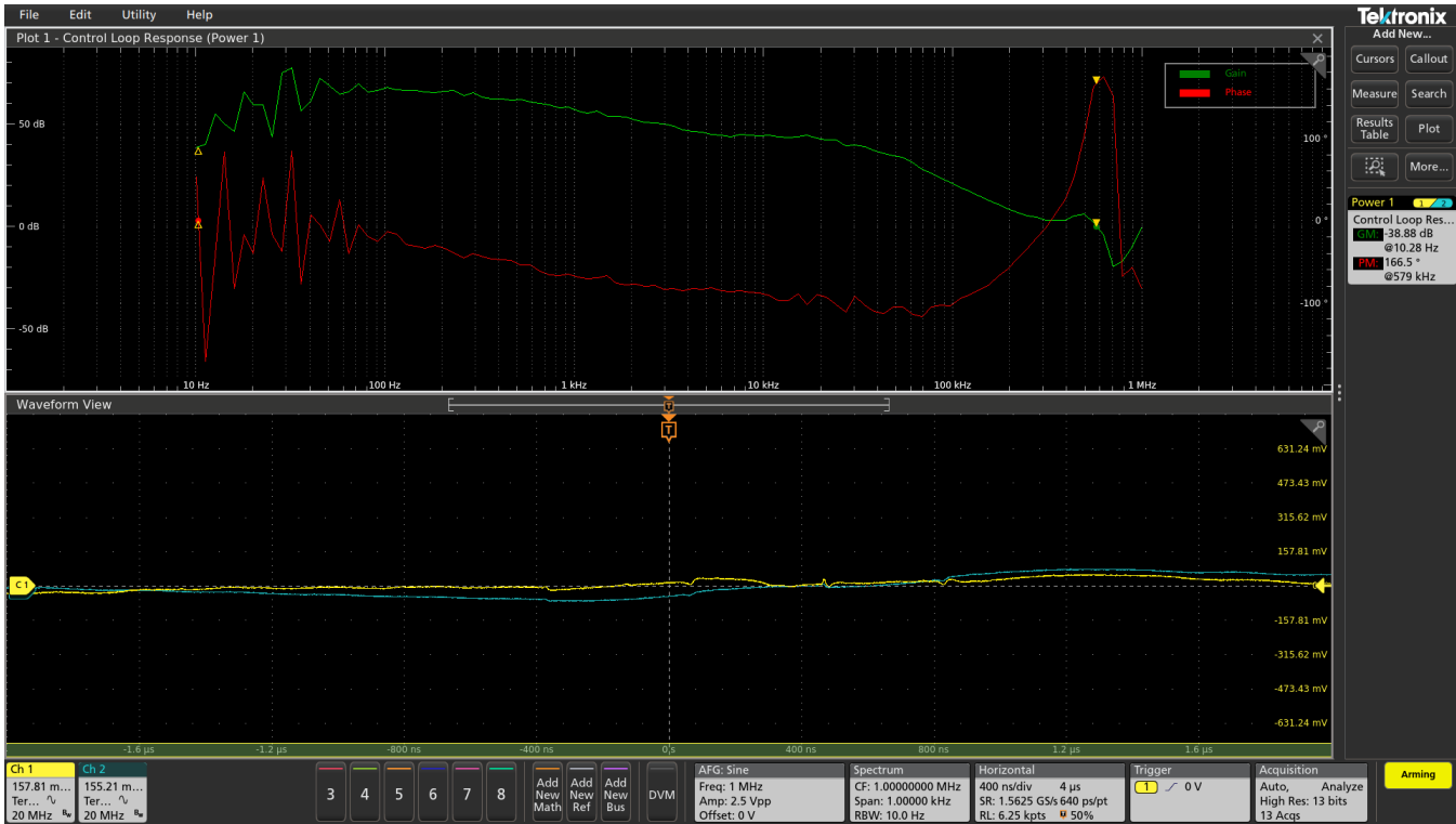
Figure 16: Control Loop Response (Bode plots) plots gain and phase versus frequency and calculates the gain margin and phase margin.
