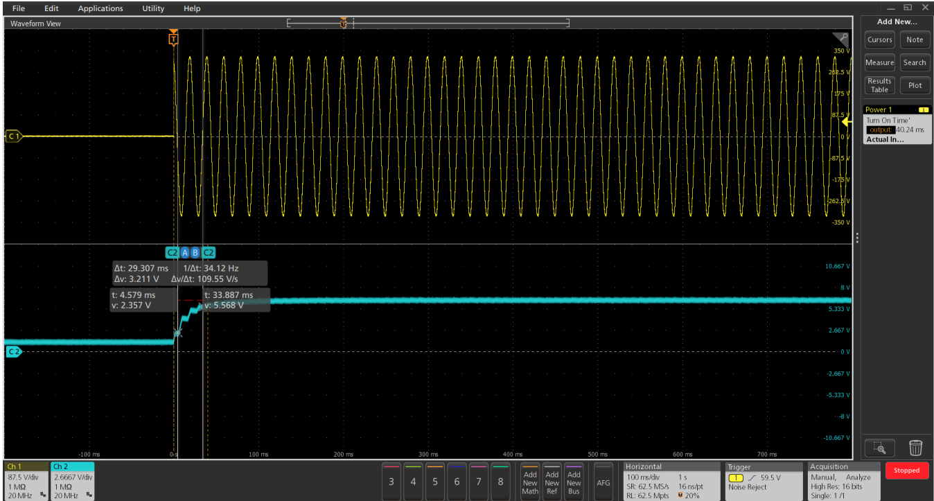
Figure 12: Turn on time measurement
