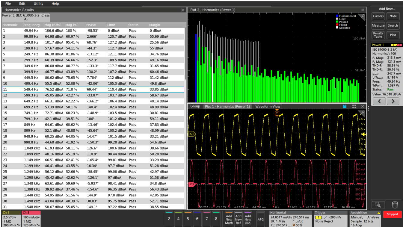
Figure 2: Harmonics bar graph, harmonics results table, and traverse capability via the results bar (upper right)
