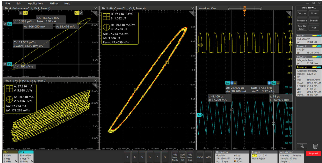
Figure 8: Magnetic Analysis measurement with B-H curve, I vs. \int V , and Inductance plots
