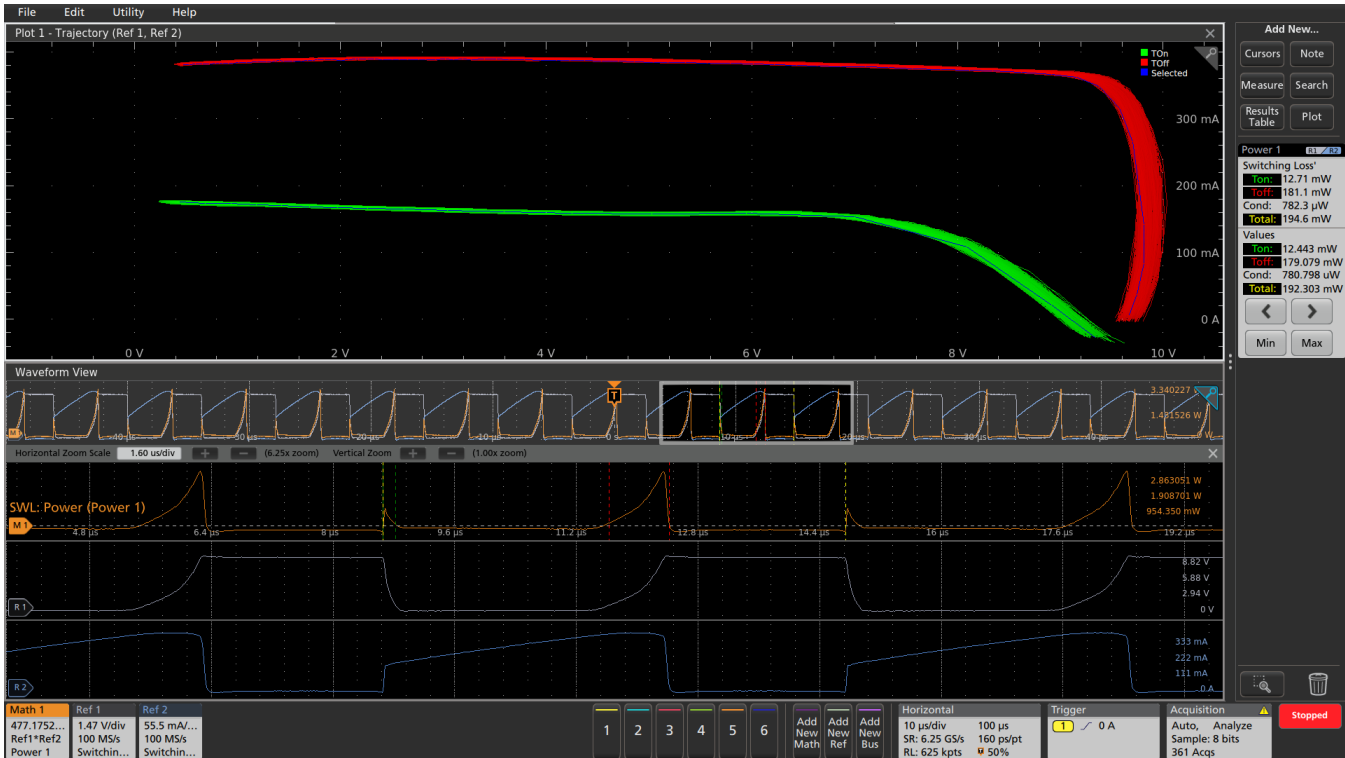
Figure 5: Switching Loss Trajectory Plots (upper window) show the T_{on} loss, and T_{off} loss for all switching cycles in a single plot.
