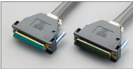
3721-MTC-3: 50-pin D-sub female to 50-pin D-sub male cable. 3 m (10 ft) length.
