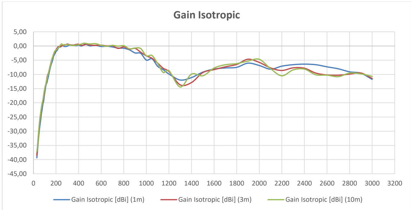
30 MHz ... 3000 MHz, Isotropic Gain of TBMA1B
