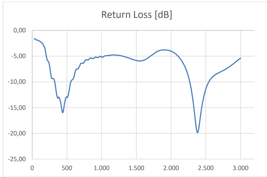
TBMA1B, S11, 30 MHz ... 3000 MHz
