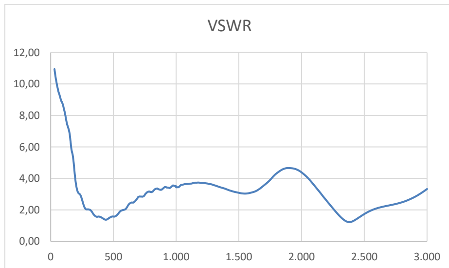
TBMA1B, VSWR, 30 MHz ... 3000 MHz
