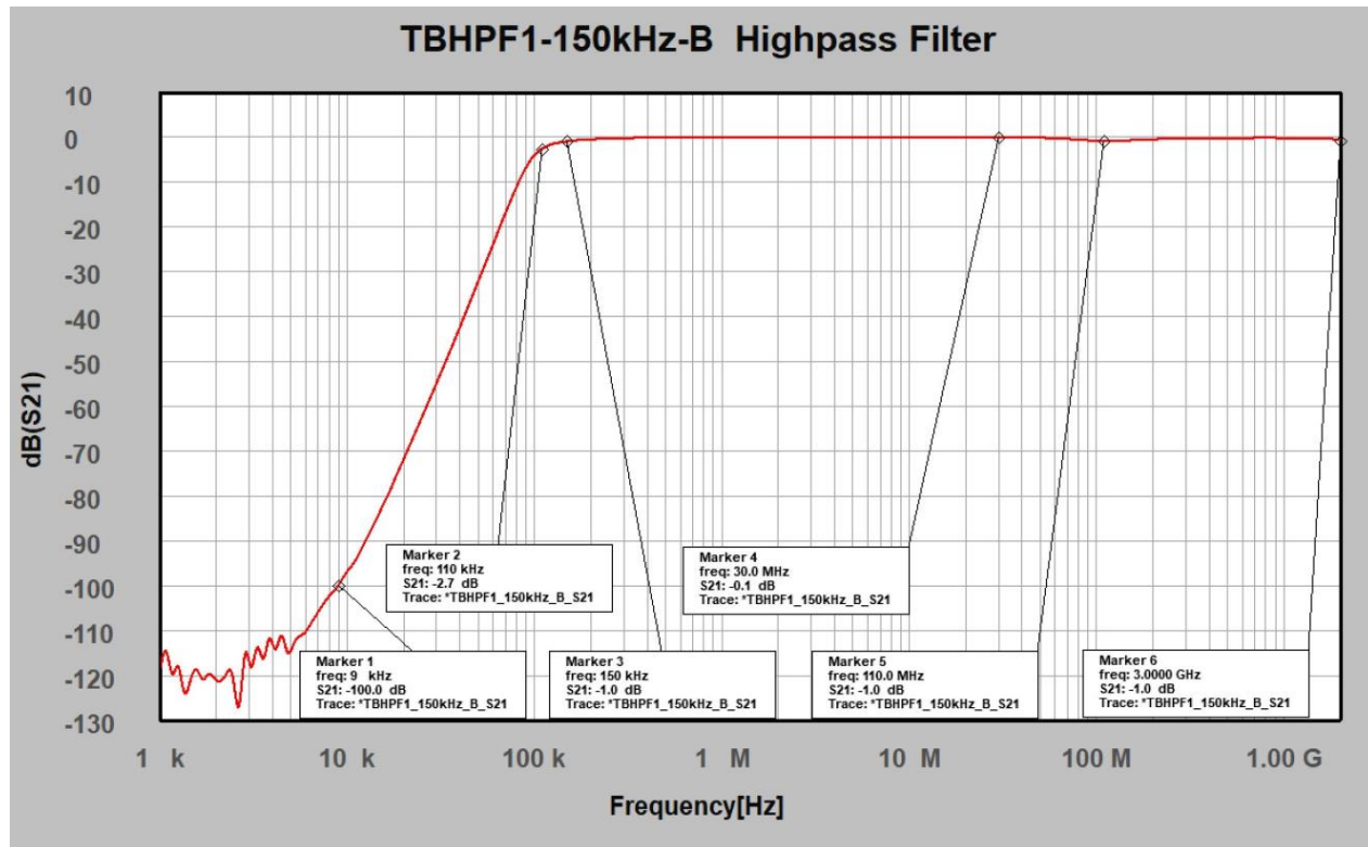
TBHPP1-150kHz-B: Insertion loss, 1 kHz to 3 GHz, typical data
