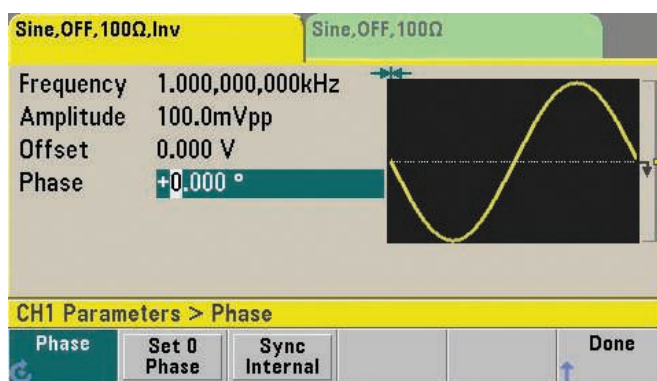
Figure 1. 33600A Series' menu for internal phase sync.
