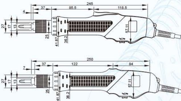
Lever Start Type ED-212L1 ~ ED-219L2
