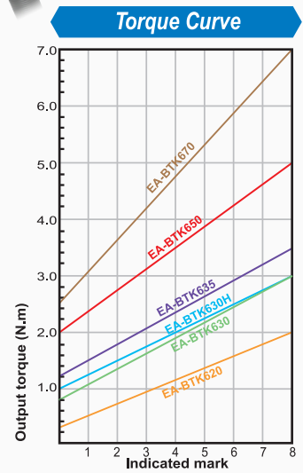
EPAA50006-B6P-6N (For BTK620~BTK670)
