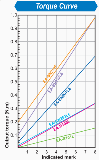
Push To Start Type EA-BN210P/CE6
