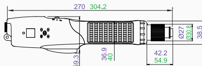
Lever Start Type EA-BD412L/CE6 ~ EA-BD419L/CE6 EA-BD630L/CE6 ~ EA-BD650L/CE6
