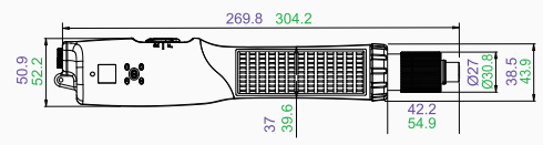
Push to Start Type EA-BD412P/CE6 ~ EA-BD419P/CE6 EA-BD630P/CE6 ~ EA-BD650P/CE6
