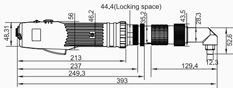
Lever Start Type EA-BAKA950L/C6 ~ EA-BAKA9220L/C6
