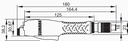
Lever Start Type EA-B101L-C/CE3 ~ EA-B103LS1-C/CE3
