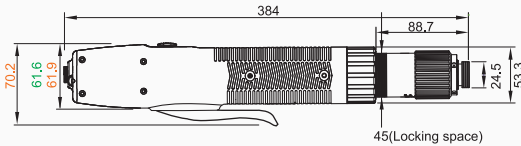
Lever Start Type EA-BAK9250LH/C6 ~ EA-BAN9500LW/C6
