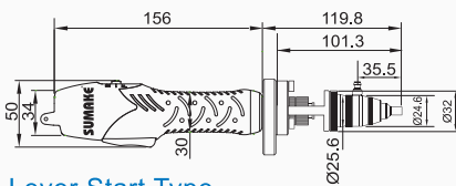
Lever Start Type EA-BN203LAS-C ~ EA-BN210LAS-C
