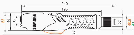
Lever Start Type EA-BN412L - EA-BN419L
