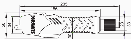
Lever Start Type EA-BN203L/CE6 ~ EA-BN210L/CE6
