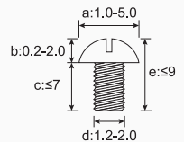
SFR20M (Manual Type)
