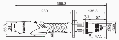
Lever Start Type EA-BN623LHAS ~ EA-BN650LAS
