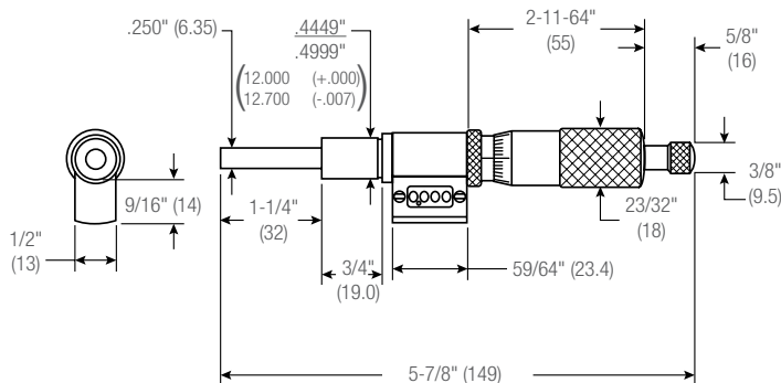
363RL (0-1") and 363MRL (0-25mm) dimensions
