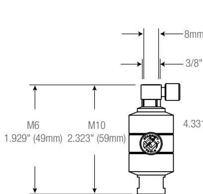
Short holder M6 and M10 with 3/8" or 8mm stem
