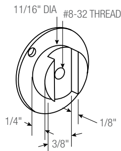
PT25157 Adjustable Bracket Back
