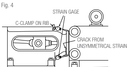
Fig. 4 STRAIN BETWEEN APPLIED ENGINE FRAME (WHILE OPERATING), DIFFERENCE BETWEEN TOP AND BOTTOM READINGS OF THE STRAIN GAGE INDICATES IMPROPER ALIGNMENT, CAUSING CRACKS.
