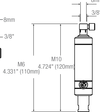
Long holder M6 and M10 with 3/8" or 8mm stem
