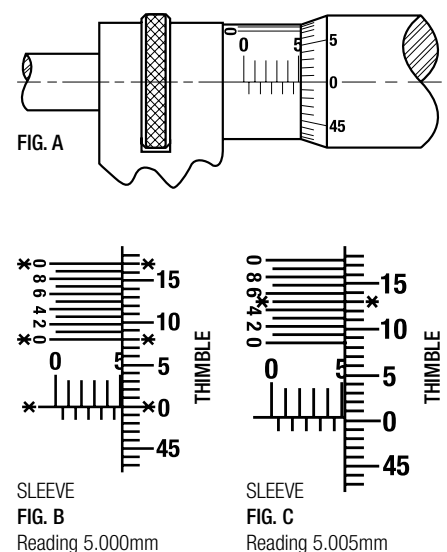
FIGURE C – READING 5.005mm
