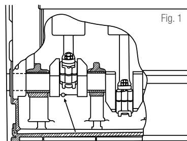
Fig. 1 STRAIN GAGE APPLIED TO CRANK OF DIESEL ENGINE TO DETERMINE IMPROPER ALIGNMENT.
