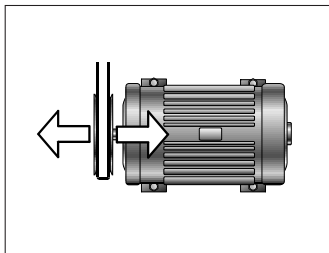
Fig 14 Parallel alignment
