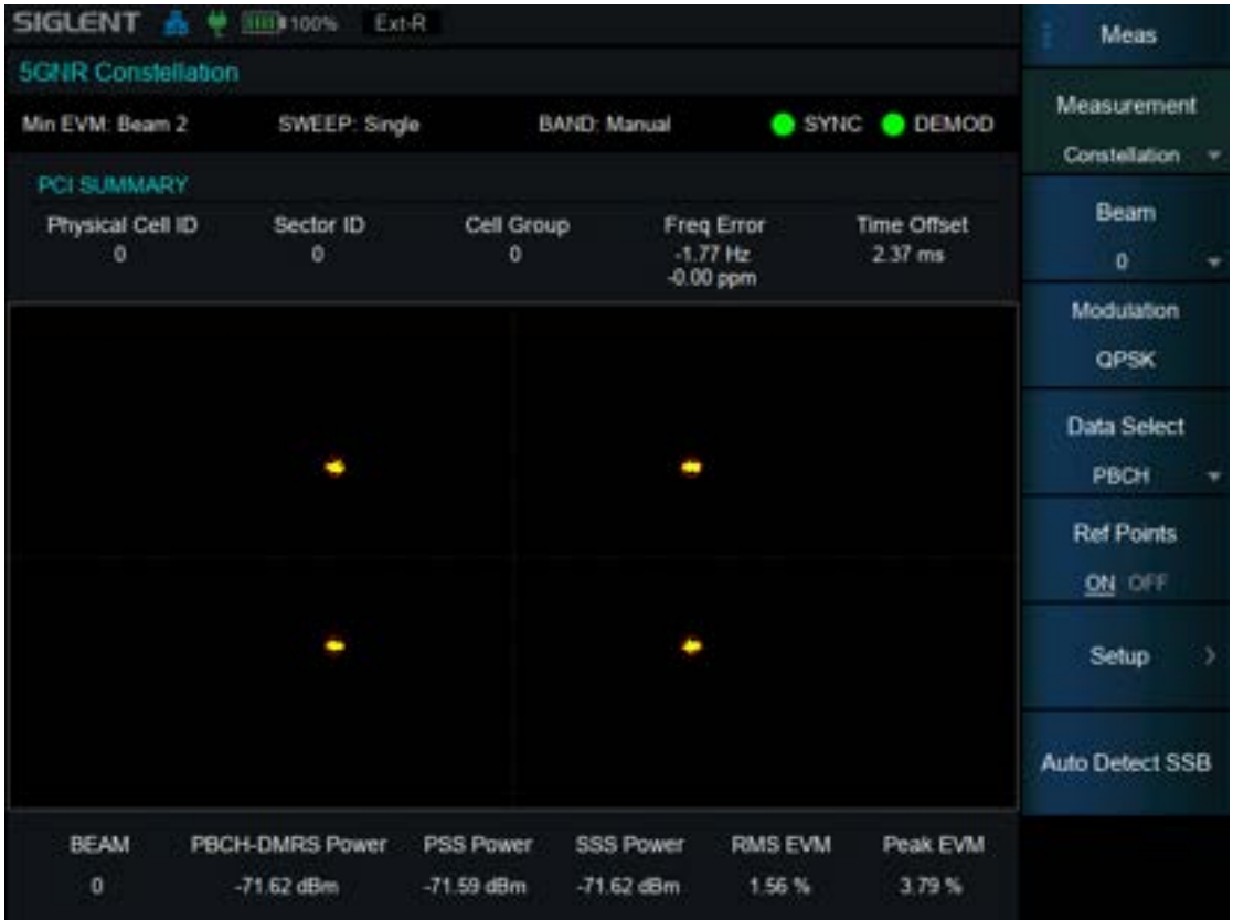
Figure 8–8 Constellation View
