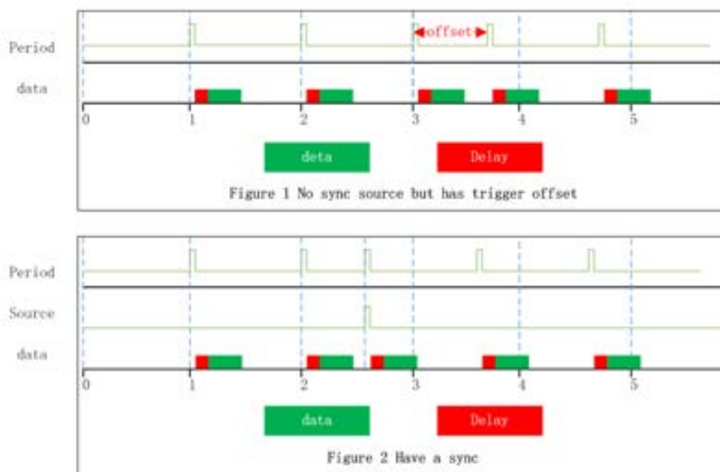
Figure 3–1 Trigger of synchronization source
