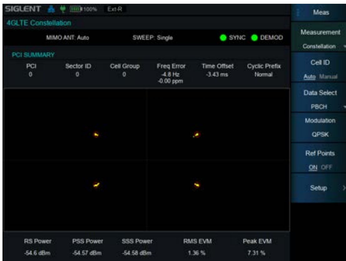
Figure 9–7 Constellation View
