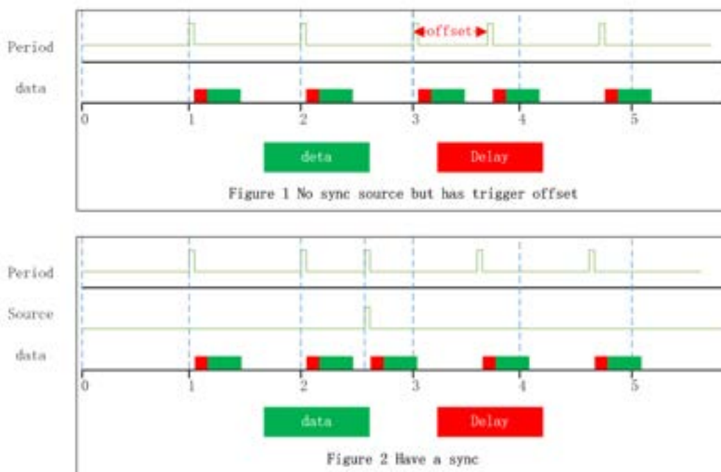
Figure 6–1 Sync Source trigger
