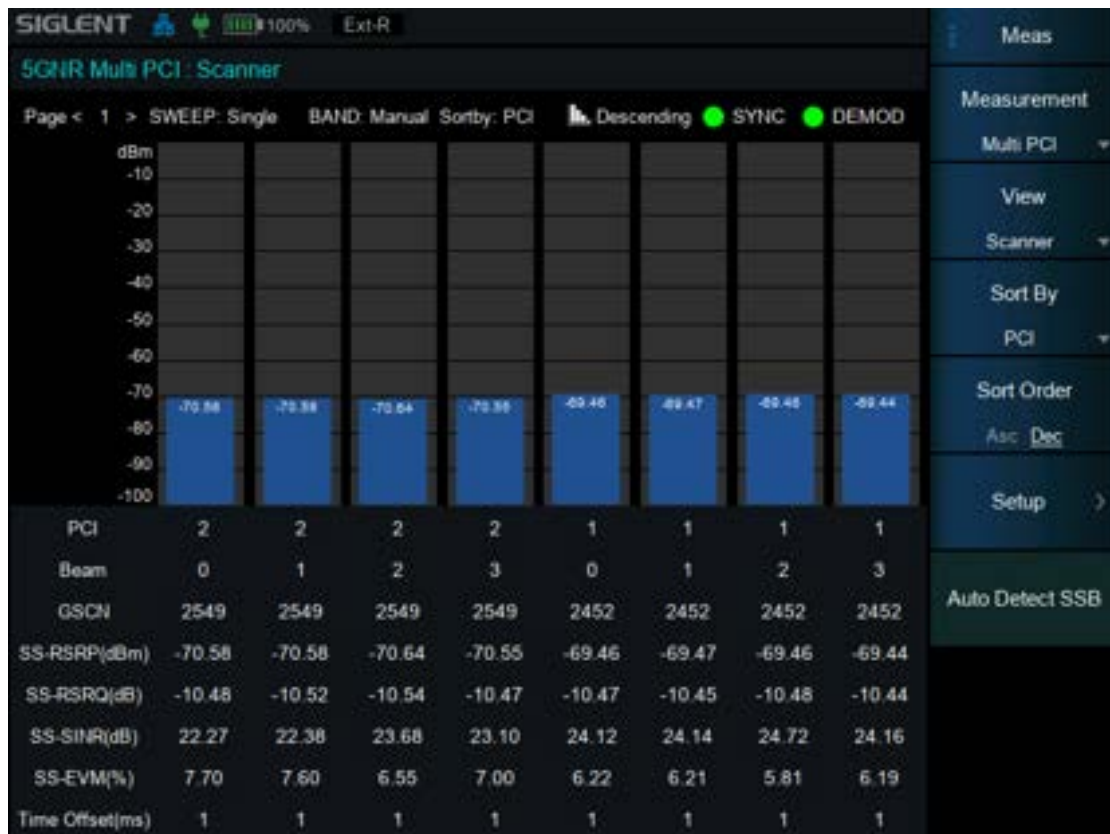
Figure 8–3 Multi-PCI histogram display
