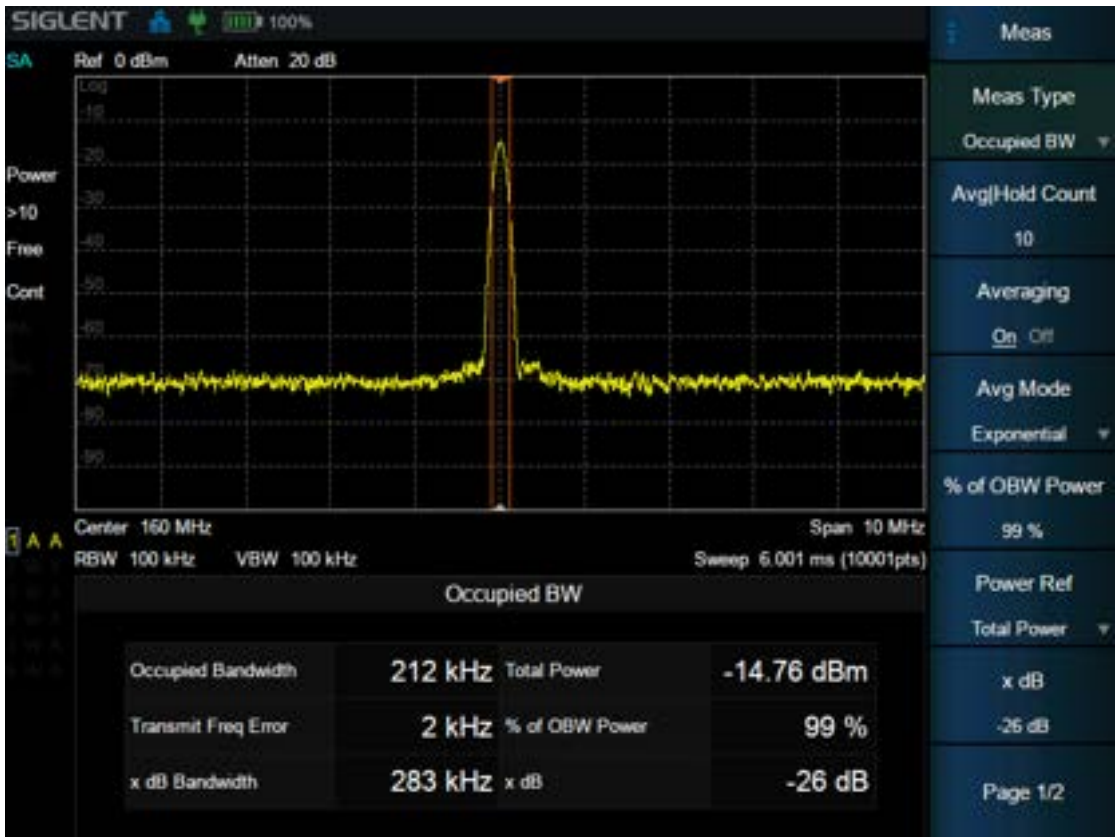
Figure 3–9 OBW
