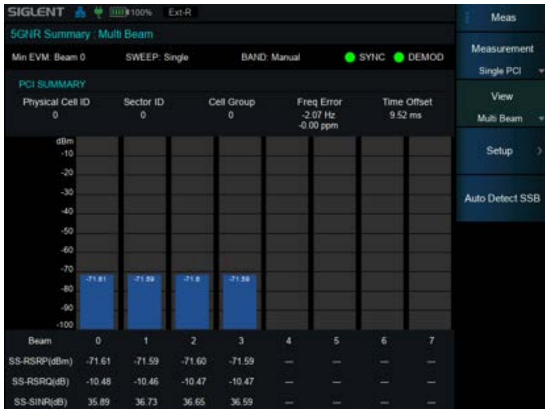
Figure 8–2 Multi Beam View
