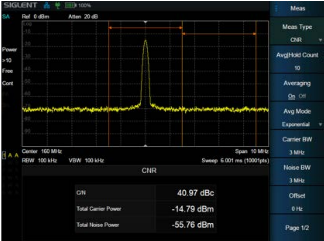
Figure 3–13 CNR
