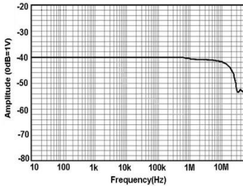
Fig 4 SCP5150 Amp- Frequency curve
