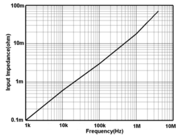
Fig 9 SCP5500 Input impedance VS Frequency
