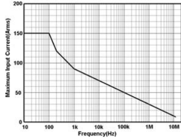
Fig 5 SCP5150 Continuous maximum input measurement
