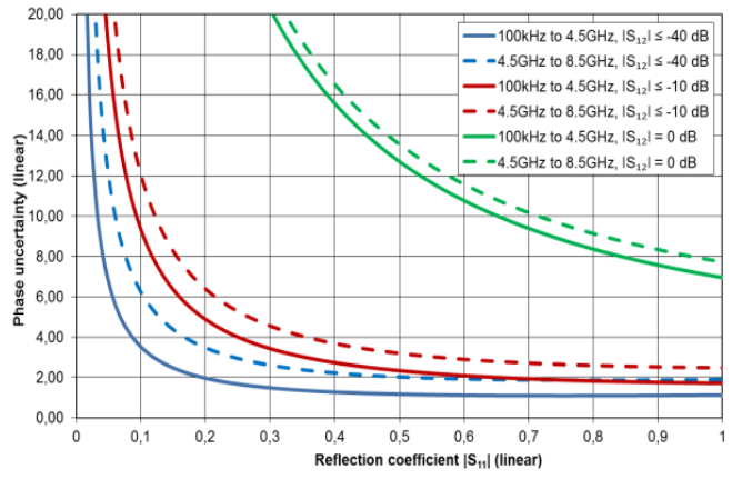
Typical accuracy of reflection magnitude and reflection phase measurements for the R&S®ZND Analysis conditions: S_{21} = 0 , cal. power -10 dBm, meas. power -10 dBm, Base unit or K1 installed.
