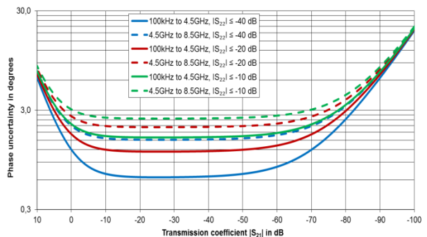
Typical accuracy of transmission magnitude and transmission phase measurements for the R&S®ZND Analysis conditions: S_{11} = 0 , cal. power -10 dBm, meas. power -10 dBm, Base unit or R&S®ZND-K1 installed.
