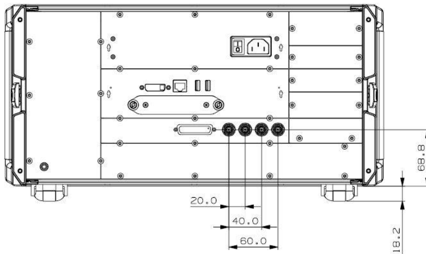
Rear view of the R&S®ZND.
