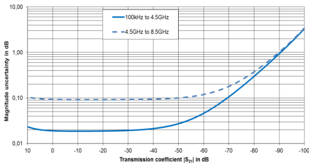
Typical accuracy of transmission magnitude and transmission phase measurements for the R&S®ZND Analysis conditions: S_{11} = S_{22} = 0 , cal. power -10 dBm, meas. power -10 dBm, R&S®ZND-K5, R&S®ZND-K6 or R&S®ZND-K8 installed.
