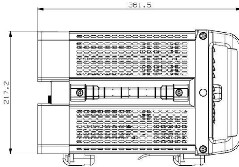
Side view of the R&S®ZND.
