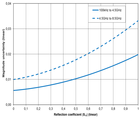
Typical accuracy of reflection magnitude and reflection phase measurements for the R&S®ZND Analysis conditions: S_{12} = S_{21} = 0 , cal. power -10 dBm, meas. power -10 dBm, R&S®ZND-K5, R&S®ZND-K6 or R&S®ZND-K8 installed.
