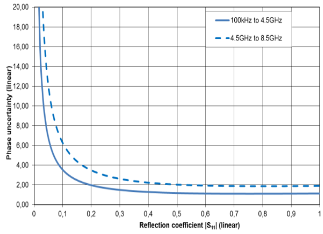
Typical accuracy of reflection magnitude and reflection phase measurements for the R&S®ZND Analysis conditions: S_{12} = S_{21} = 0 , cal. power -10 dBm, meas. power -10 dBm, R&S®ZND-K5, R&S®ZND-K6 or R&S®ZND-K8 installed.
