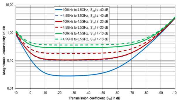
Typical accuracy of transmission magnitude and transmission phase measurements for the R&S®ZND Analysis conditions: S_{11} = 0 , cal. power -10 dBm, meas. power -10 dBm, Base unit or R&S®ZND-K1 installed.
