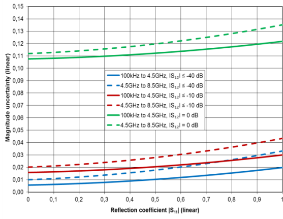
Typical accuracy of reflection magnitude and reflection phase measurements for the R&S®ZND Analysis conditions: S_{21} = 0 , cal. power -10 dBm, meas. power -10 dBm, Base unit or K1 installed.
