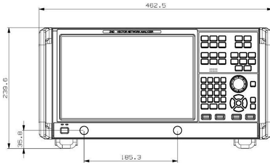
Front view of the R&S®ZND.
