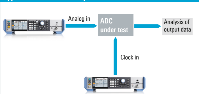
ADC test setup with two R&S®SMA100B as the signal sources for the analog input and for the clock input.
