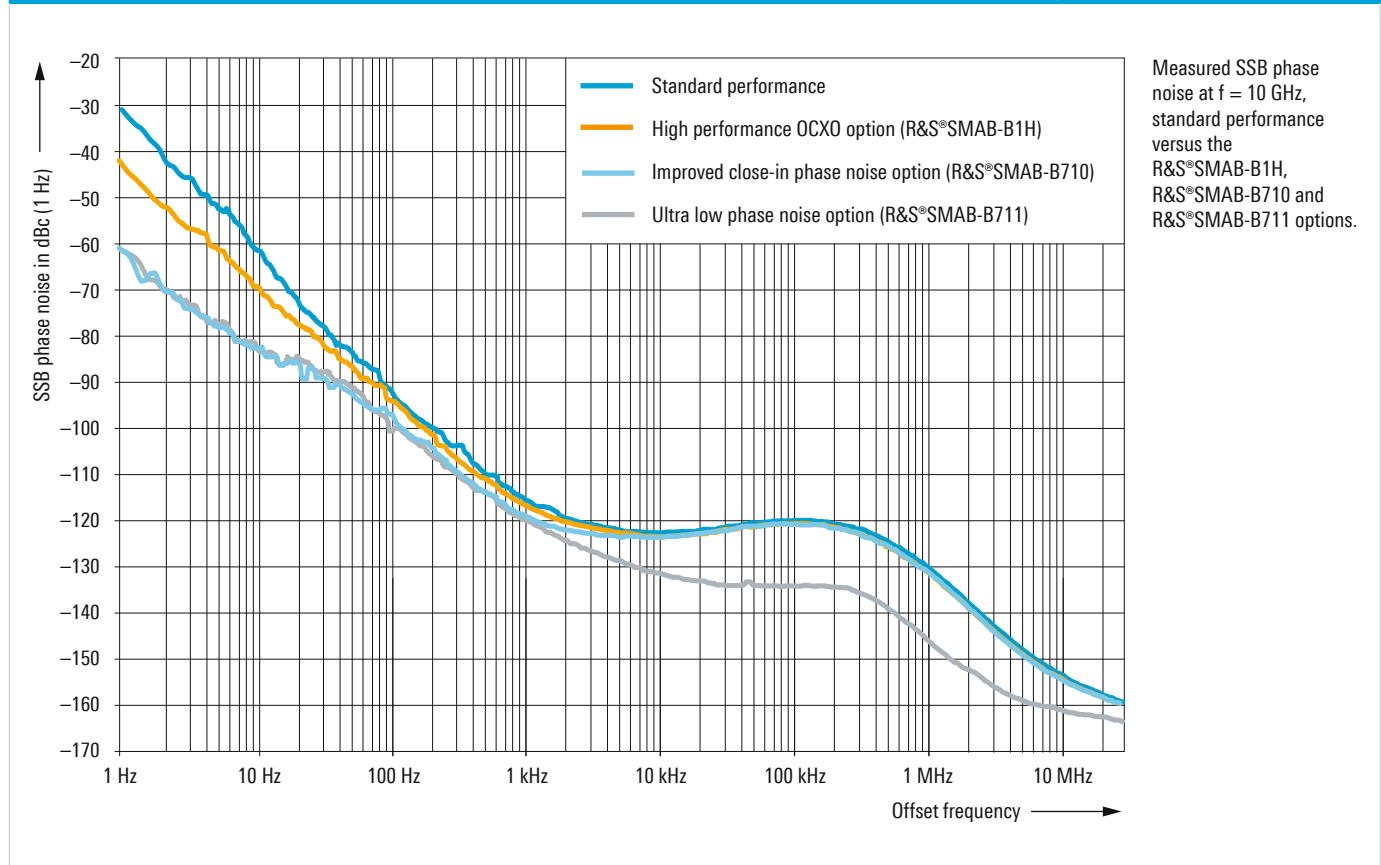
Measured SSB phase noise performance of the R&S®SMA100B for X-band radar signal
