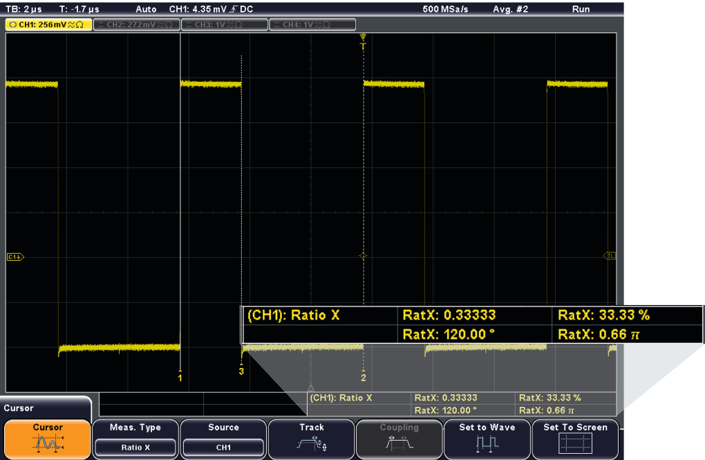
Special cursor measurement: using three cursors to determine the duty cycle of a pulsed signal.
