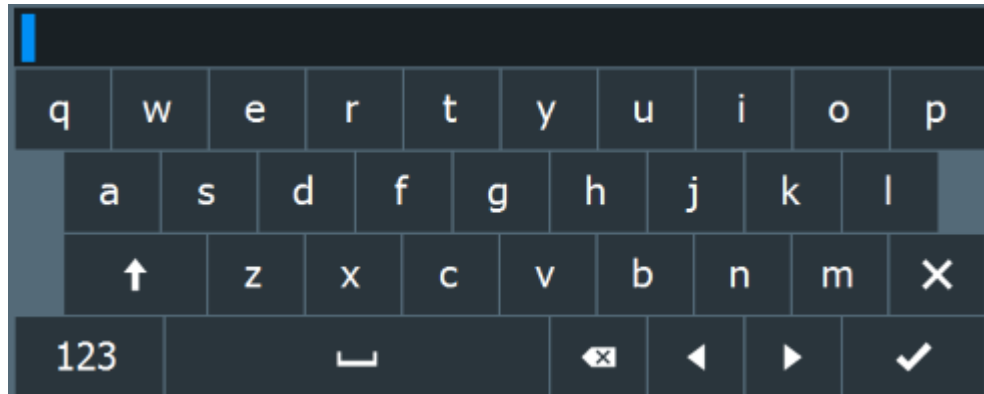
Figure 4-5: Alphanumeric editor
