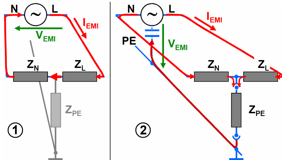
Figure 4-42: 2-line LISN in differential mode (1) and in common mode (2)
