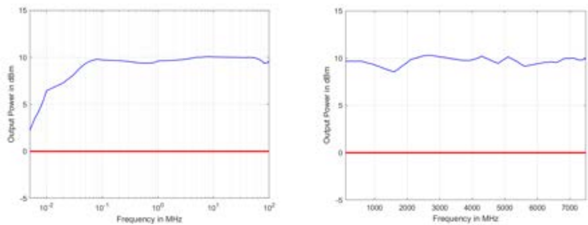
Maximum output power versus frequency, level in dBm (meas.)
