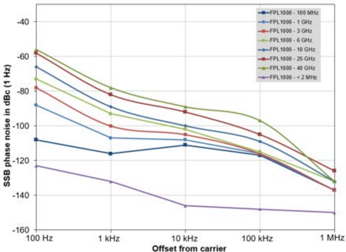
Measured SSB phase noise at different center frequencies
