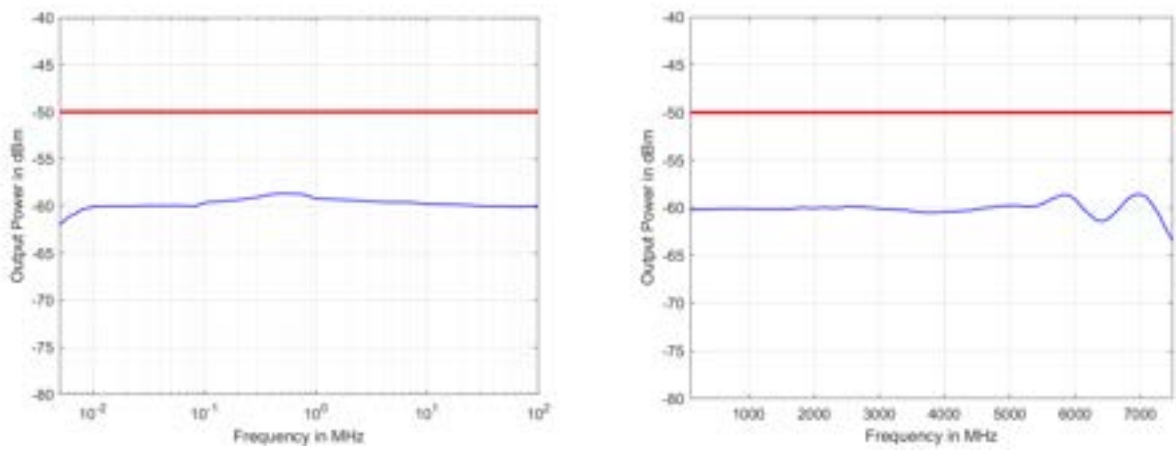
Minimum output power versus frequency, level in dBm (meas.)
