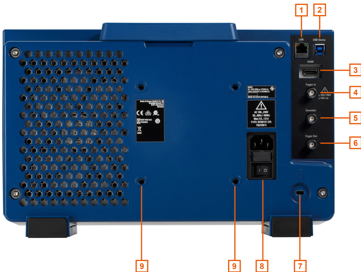
Figure 5-3: Rear panel view of MXO 3
