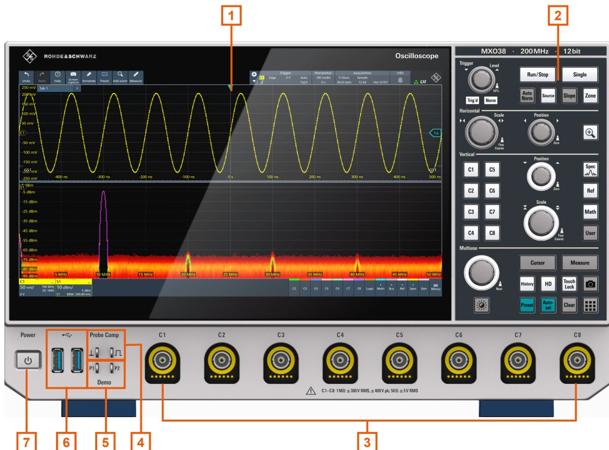
Figure 5-1: Front panel of an 8-channel MXO 3
