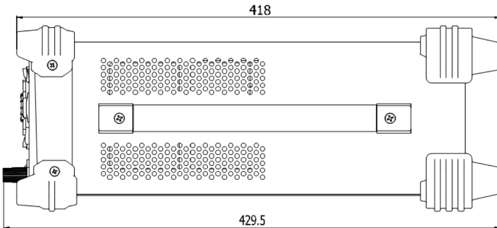
Figure 2 Side View
