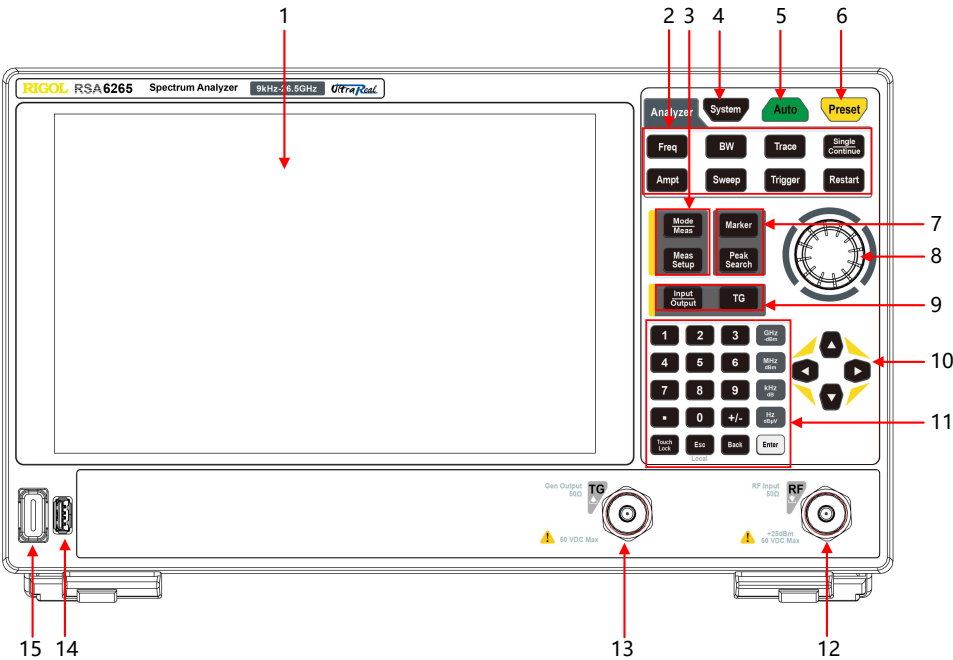
Figure 3.1 Front Panel
