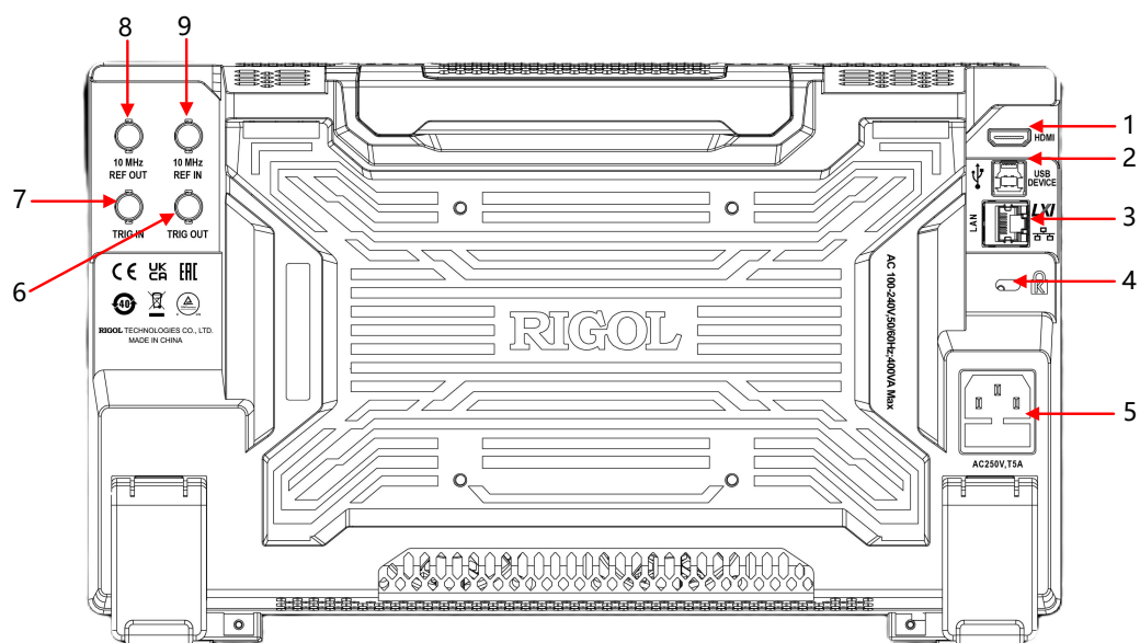
Figure 3.2 Rear Panel
