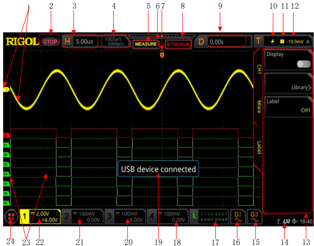
Figure 4.15 User Interface
