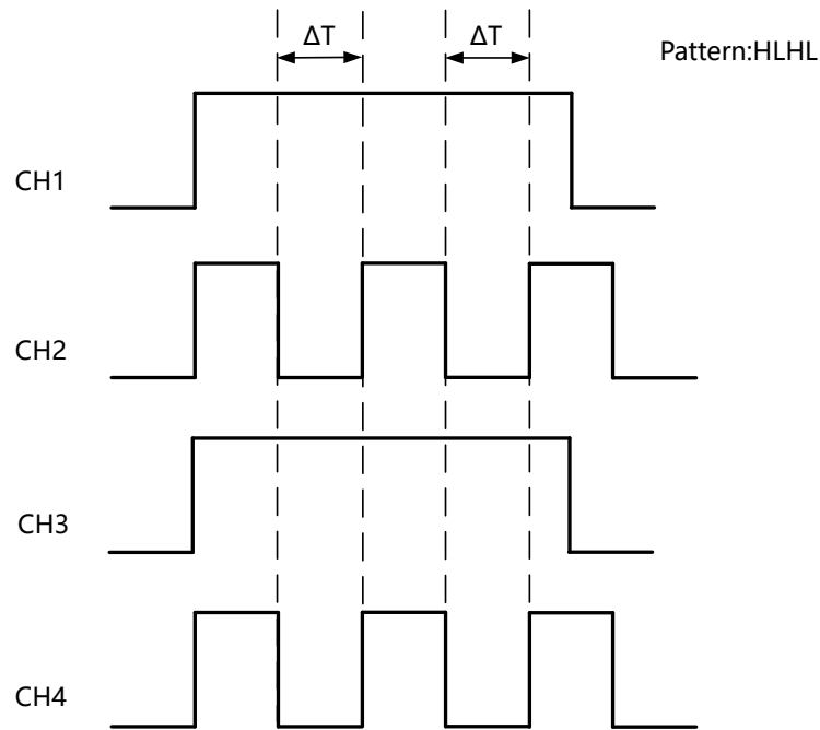
Figure 8.7 Duration Trigger
