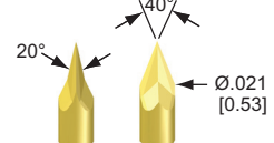
9R-S - Razor
