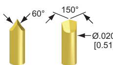
8R-S - Razor
