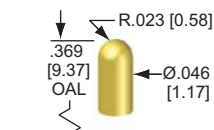
40 - Round
