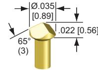
03-S - Chisel .045 [1.14] Min. Centers
