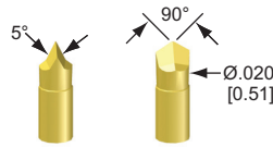
6R -S - Razor
