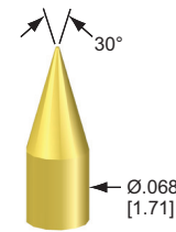
41 - Spear
