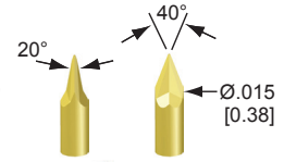
9R -S- Razor
