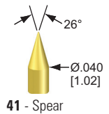
41 - Spear
