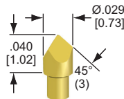
13-S - Chisel .232 [5.89] Full Stroke
