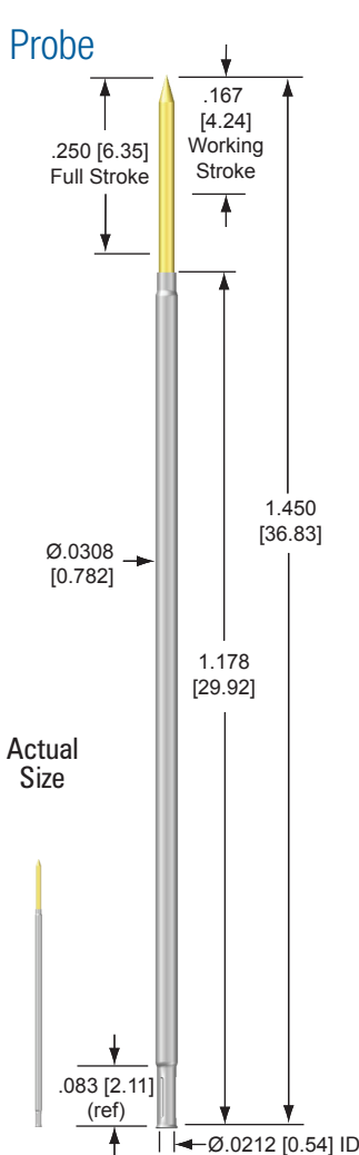
03 or 03-S - Chisel .045 [1.14] Min. Centers
