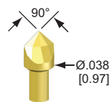
71 -S- Blade
