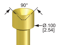
22 - Cup
