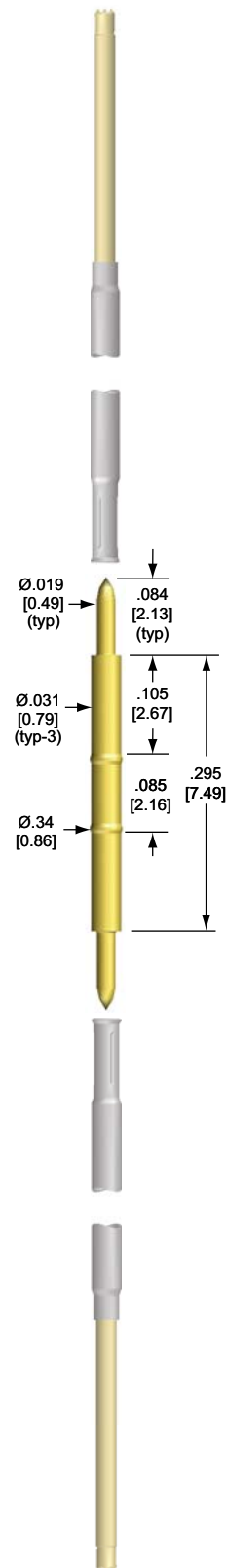
Termination P/N: X39-TX-3G
