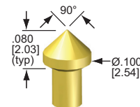
01 - Spear
