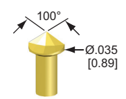
51-S - Blade .045 [1.14] Min. Centers
