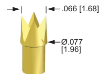
24 - Crown
