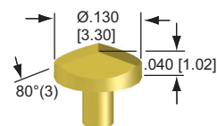
33 - Chisel .150 [3.81] Min. Centers
