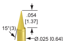
53 or 53 -S- Chisel
