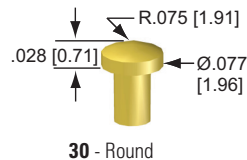
30 - Round
