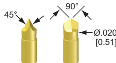
6R-S - Razor
