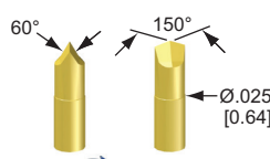
8R -S- Razor
