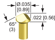
03 or 03-S - Chisel .045 [1.14] Min. Centers
