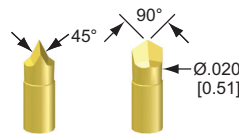
6R-S - Razor
