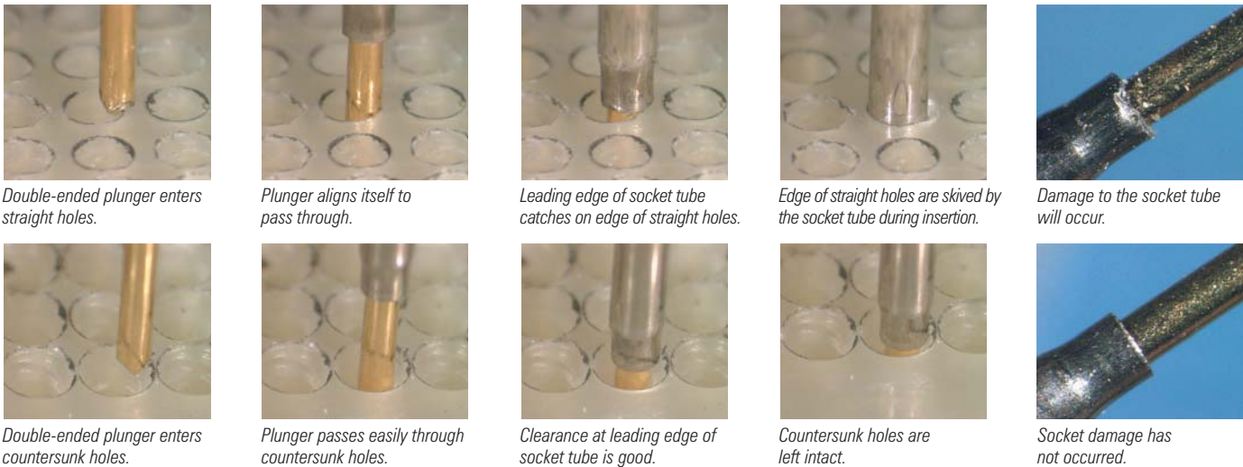
Advantage of using countersunk holes vs straight holes guide plates.
