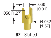
62 - Slotted
