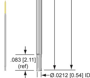
13-S - Chisel .232 [5.89] Full Stroke
