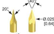
9R -S- Razor
