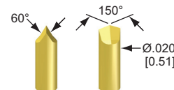
8R-S - Razor
