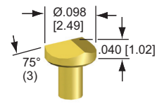
23 - Chisel .120 [3.05] Min. Centers
