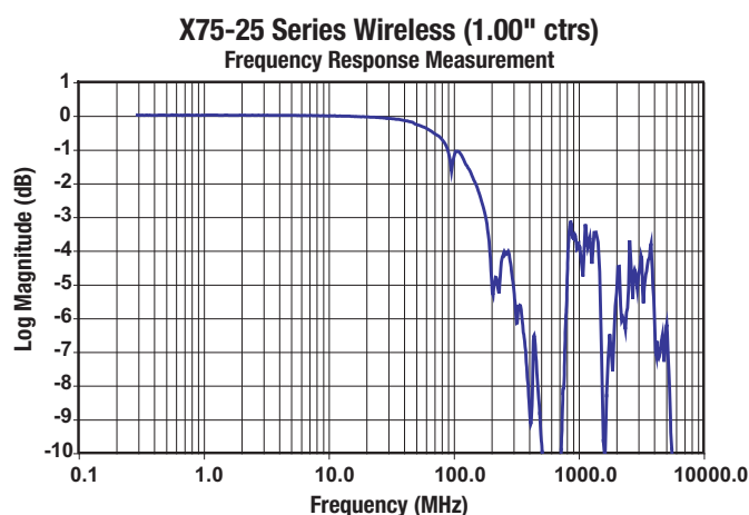
Diagram A: Frequency response of two .075 [1.91] wireless X Probes (signal and ground) on 1.00 [25.4] centers.
