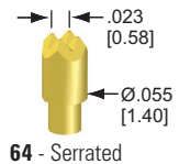
64 - Serrated
