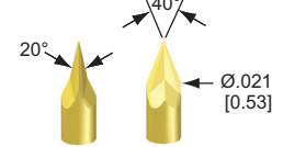
9R-S - Razor
