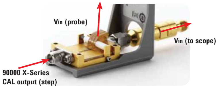
Figure 5: Depiction of V_{in}/V_{out} as connected to the InfiniiMax III Performance Verification kit
