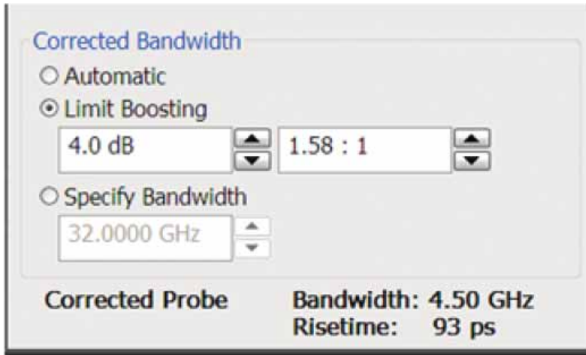
Figure 11: PrecisionProbe provides the ability to make the tradeoff between higher bandwidth and higher noise
