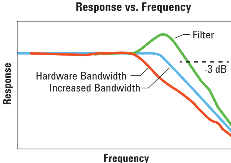
Figure 10: The effect of bandwidth-enhancement on noise
