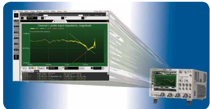
Figure 1: Characteristic of Agilent’s solder in probe impedance plot as taken by PrecisionProbe software (N2809A)
