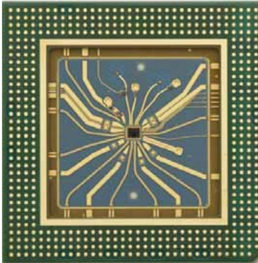
Figure 6: Agilent's custom calibration edge is enabled by the multi-chip module and Agilent's custom Indium Phosphide technology.
