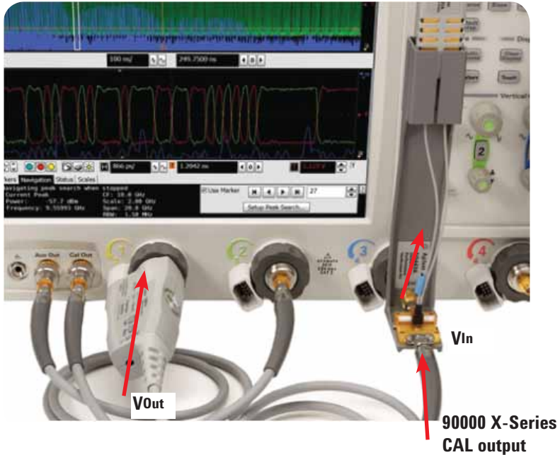
Figure 4: V_{out} as defined to the oscilloscope
