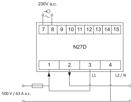
Fig. 3. Electrical connections of the PCE-N27D meter
