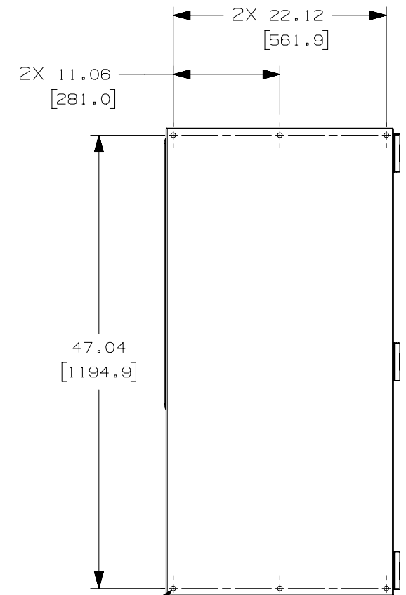
BACK VIEW
