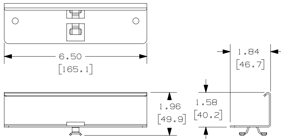
STRUT BRACKET
