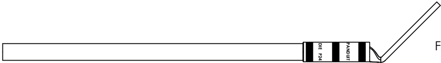
FACTORY CRIMPED #6 AWG/16mm SQ. COMMON BONDING NETWORK (CBN) JUMPER WIRE ASSEMBLY (QTY. 1) INCLUDES: LCC6-14JAWH (QTY. 1) #6 AWG/16mm SQ. WIRE - GREEN/YELLOW INSULATION 60" LONG
