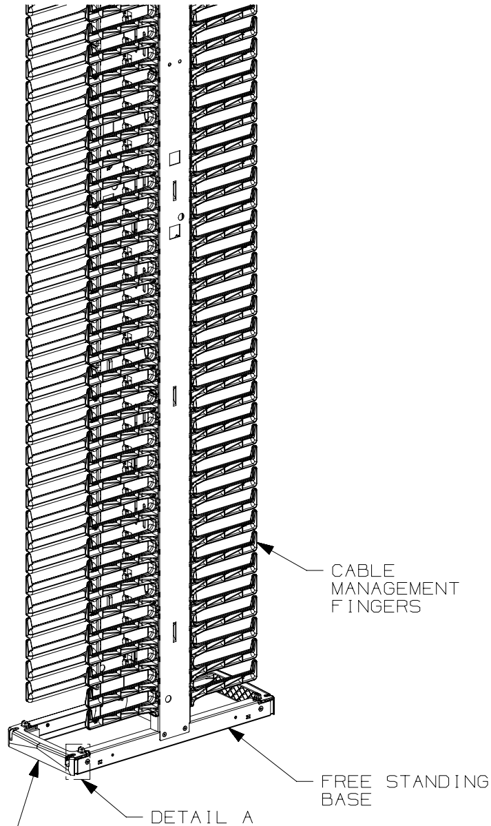
CABLE MANAGER SHOWN WITHOUT DOOR
