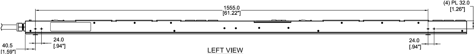
LEFT VIEW
