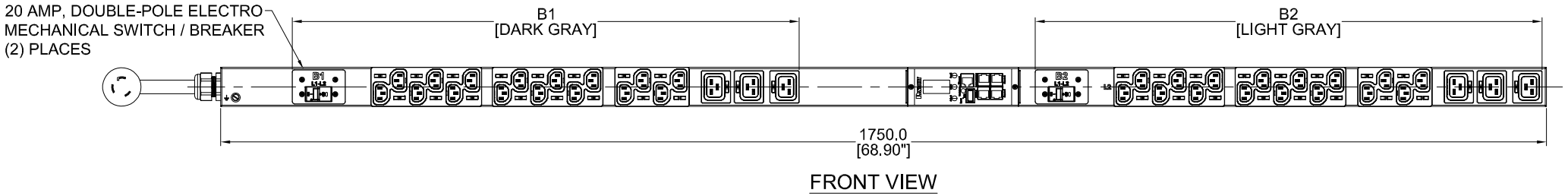
FRONT VIEW
