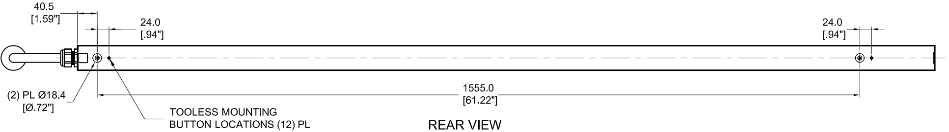
REAR VIEW
