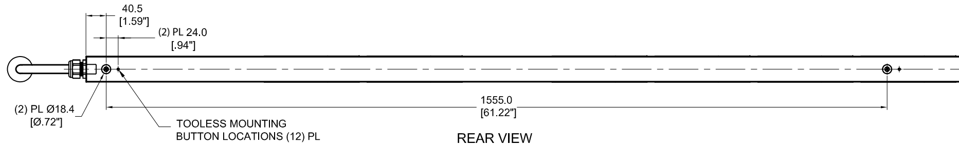
REAR VIEW
