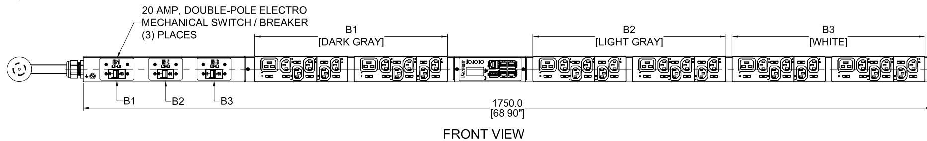
RIGHT VIEW
