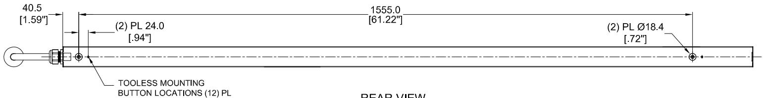
REAR VIEW
