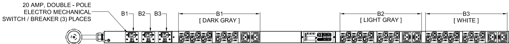
RIGHT VIEW
