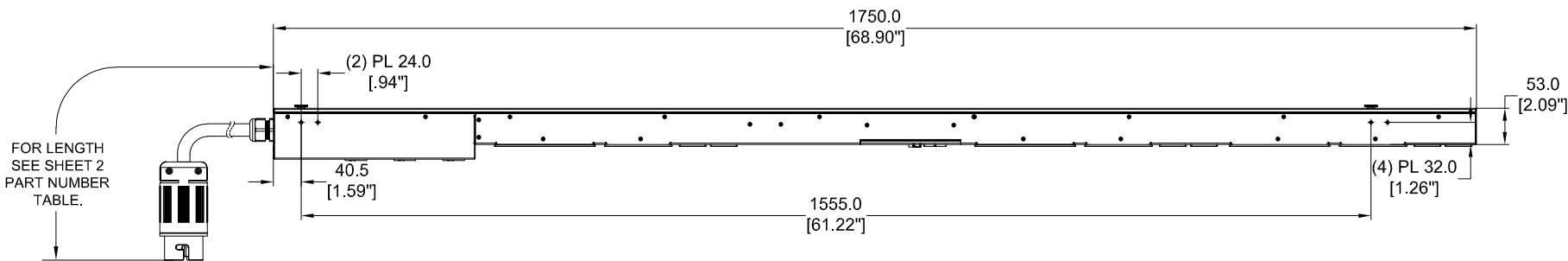
RIGHT VIEW
