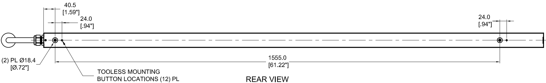
REAR VIEW
