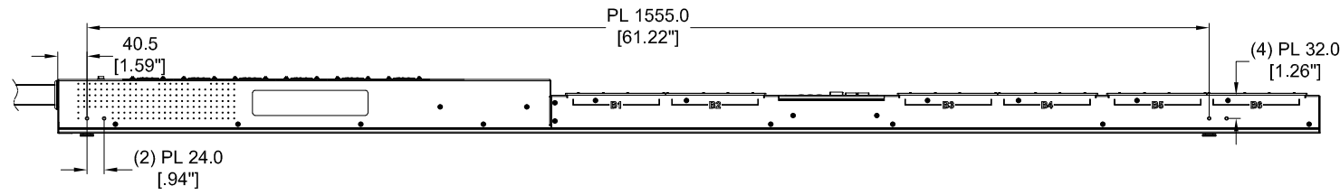
LEFT VIEW
