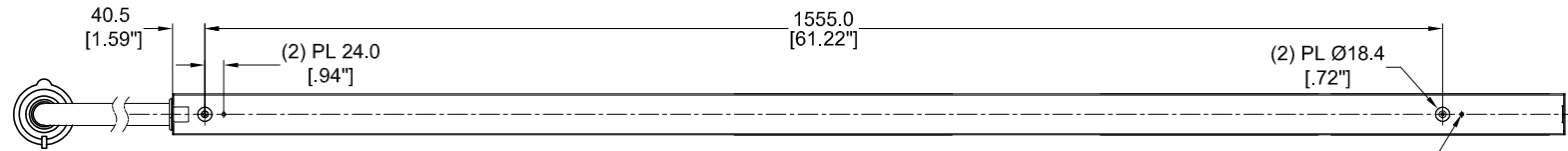
REAR VIEW
