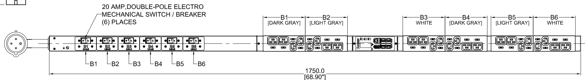
FRONT VIEW
