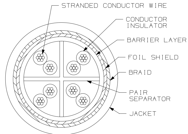
CROSS-SECTIONAL VIEW OF CABLE
