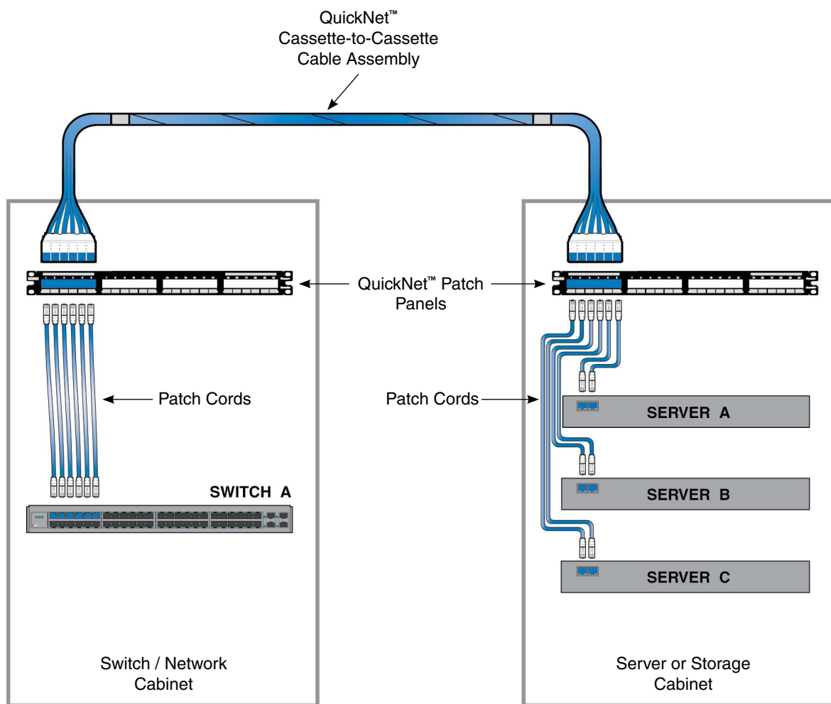
Figure 1 - Two-Connector Interconnect
