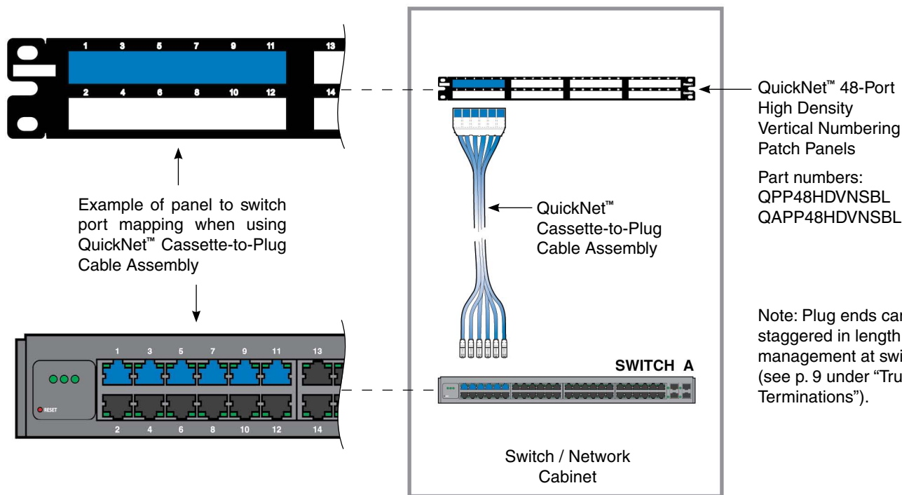
Figure 4b - QuickNet™ Cassette-to-Plug Cable Assembly
