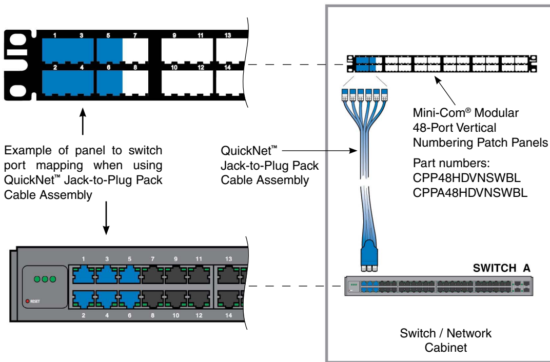
Figure 4c - QuickNet™ Jack-to-Plug Pack Cable Assembly
