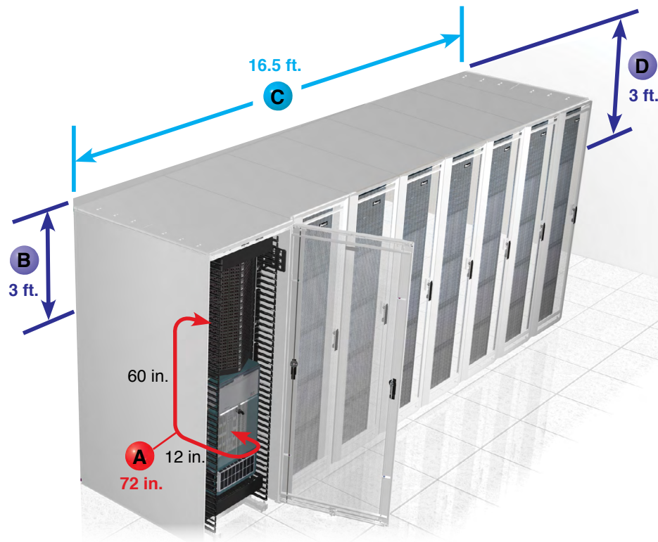
Figure 13: Measurement Example
