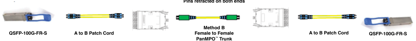
Figure 8: 10/40/100 Channel Path
