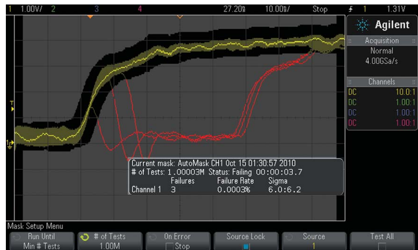
Figure 6: Mask testing to 6.2 \sigma resolution takes only seconds using an InfiniiVision scope with a mask test rate of 270,000 waveforms tests per second
