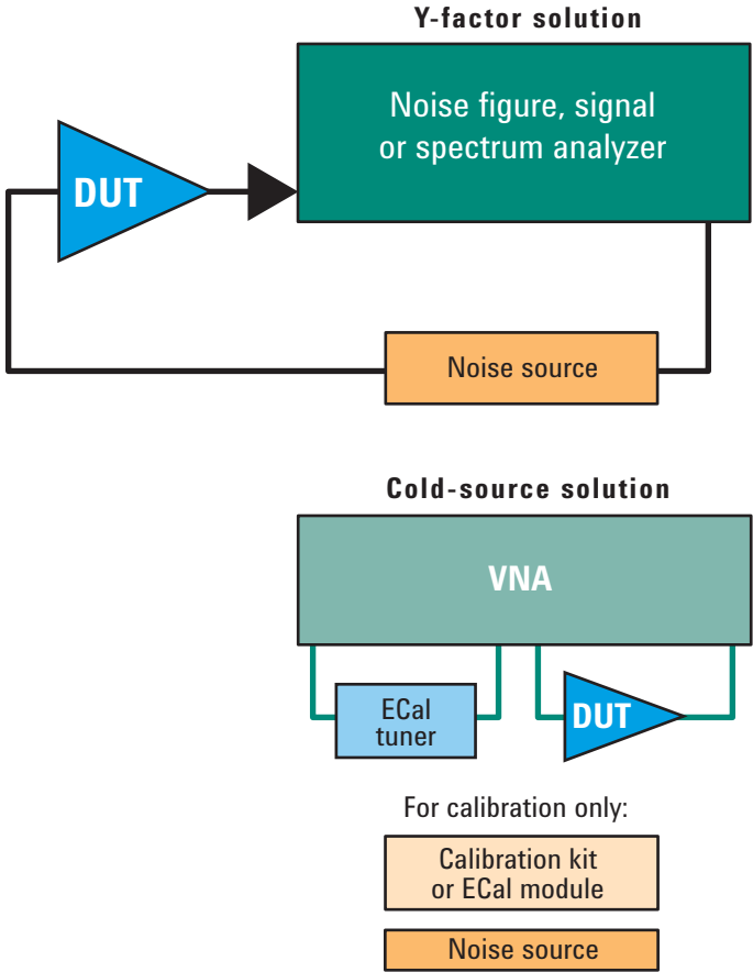
Figure 2. Basic components needed to make noise figure measurements
