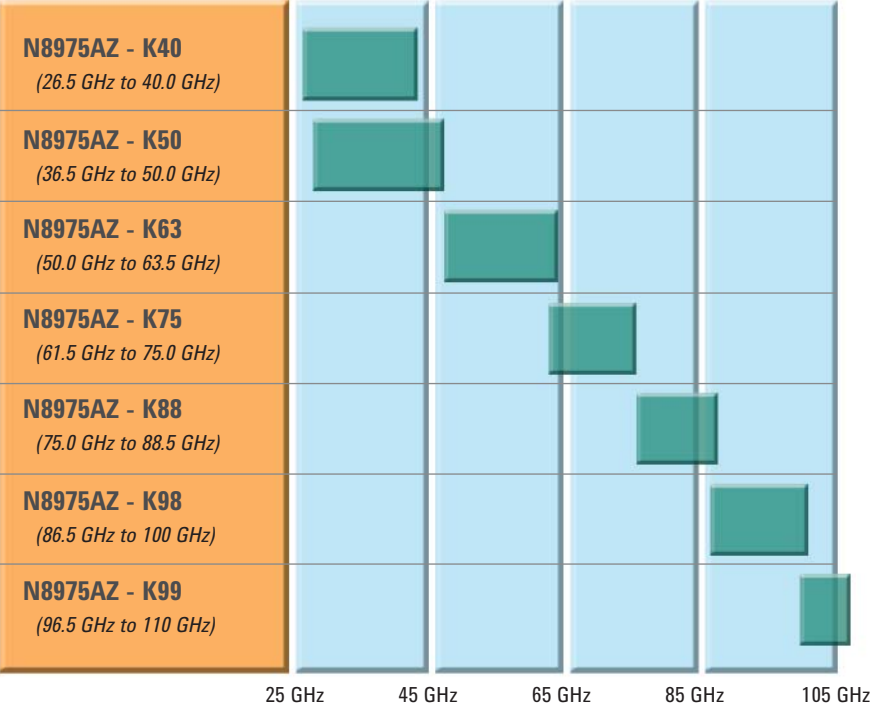
Figure 4. K-Series block downconverter frequency range chart
