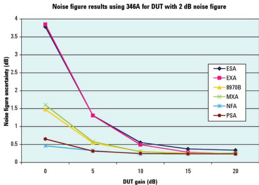
Figure 3. As the gain of a DUT decreases, Y-factor noise figure measurement uncertainty increases; below 10 dB of gain, there are significant differences between the various instrument choices
