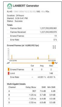
LANBERT Media Qualification app measuring available bandwidth
