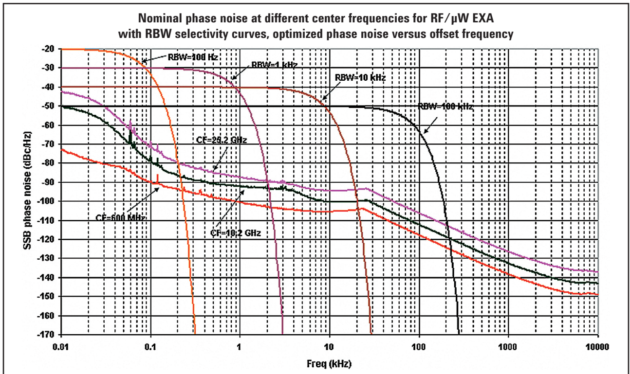
Figure 3. Nominal phase noise at different center frequencies for RF/MW EXA (Option 503, 507, 513, or 526) with SN prefix \geq MY/SG/US5340 that ships standard with N9010A-EP3.
