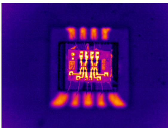
Figure 13: Same unpowered resistor as in Figure 12 but captured with a Fluke 25 micron macro lens.
