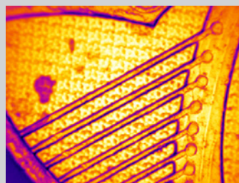
Figure 7. This image shows the same penny shown in Figure 6, captured here with a Fluke TiX560 and 25 micron macro lens. This demonstrates the very fine detail provided by the macro lens.
