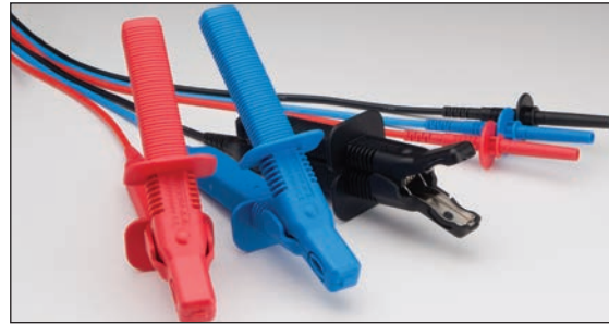
High quality flexible silicon insulated test leads with test clips meet IEC 61010. (Large clips shown.)
